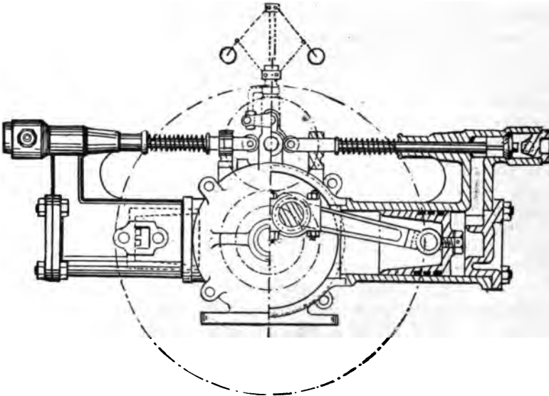
FIG. 374.—One Model of Serpollet Single-acting Two-cylinder Engine. As may be seen, this engine, with cam-actuated poppet valves, centrifugal governor for regulating the cam movement, and large fly wheel, closely resembles gas engines of the double-opposed cylinder type.
